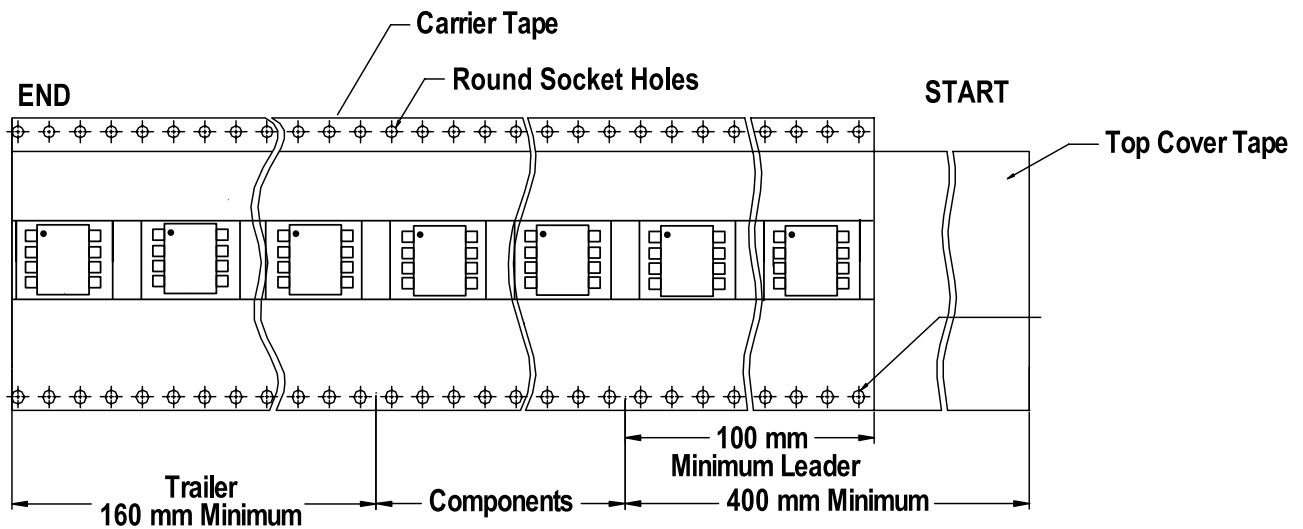
Figure 1: Tape Leader and Trailer Data
